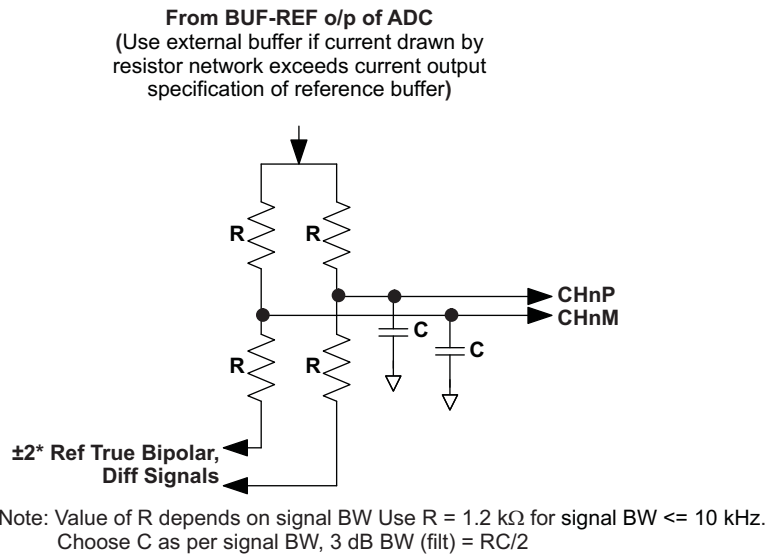
Figure 70. Bipolar Input Signals to Unipolar Differential Signals Conversion
